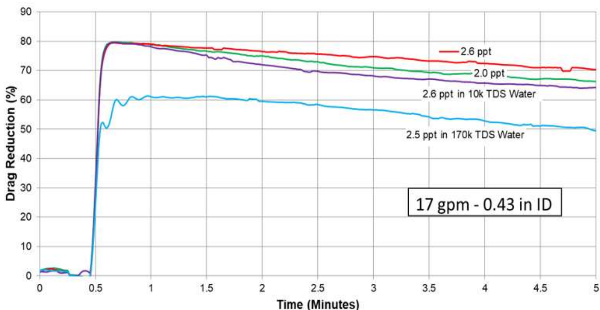
Fig 1. Friction Fighter-HB-S Flow Loop Performance in Various Water at 2-2.6 ppt Loadings
