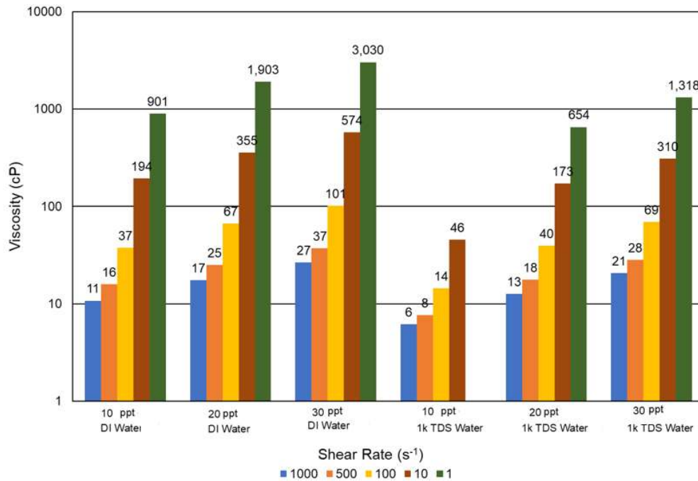
Fig 3. Friction Fighter-HB-S Viscosity Profiles in DI and 1k TDS Water
